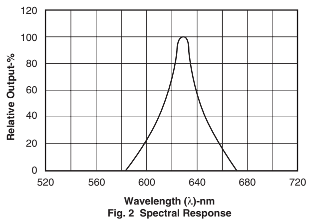
Fig. 2 Spectral Response
