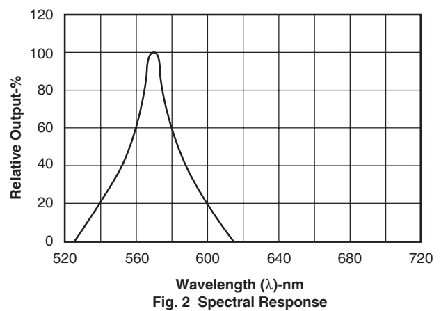
Fig. 2 Spectral Response
