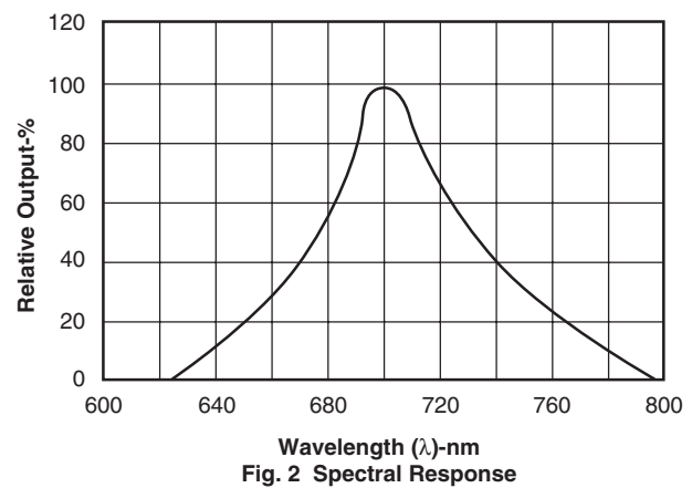
Fig. 2 Spectral Response
