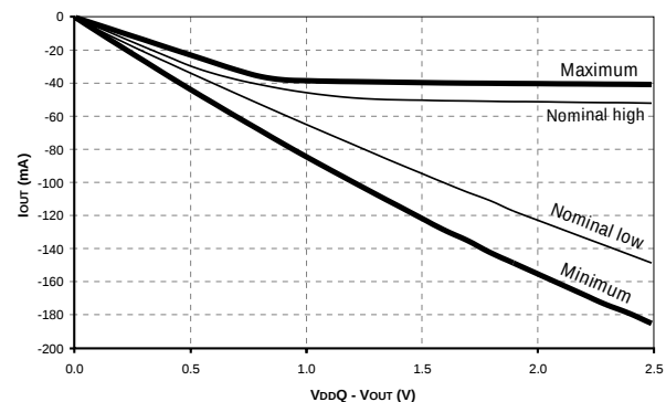
Figure 9: Pull-Up
