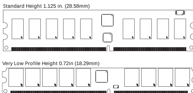
Figure 1: 184-Pin DIMM (MO-206)
