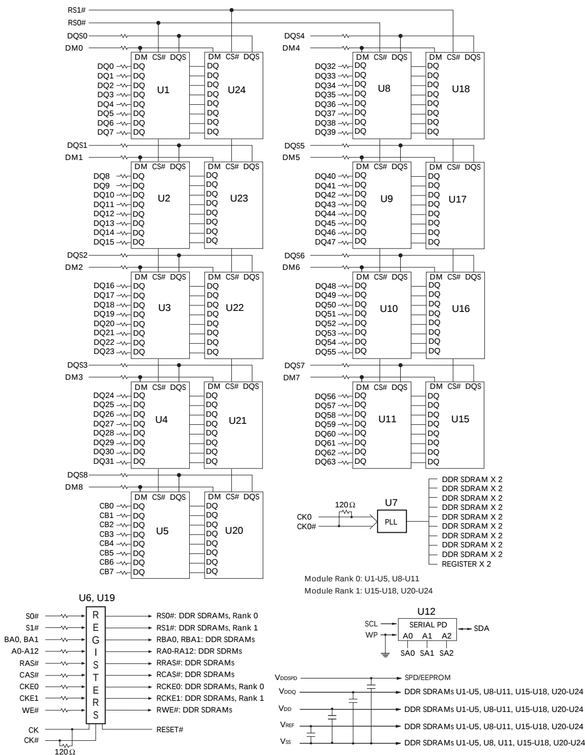
Figure 3: Standard DIMM Functional Block Diagram
