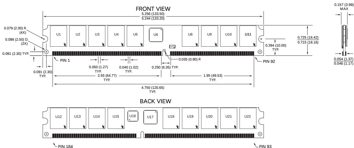
Figure 17: 184-Pin Very Low Profile DIMM Dimensions
