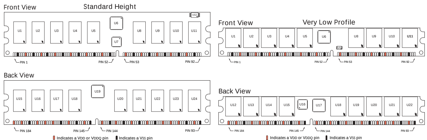
Figure 2: 184-Pin DIMM Pin Locations
