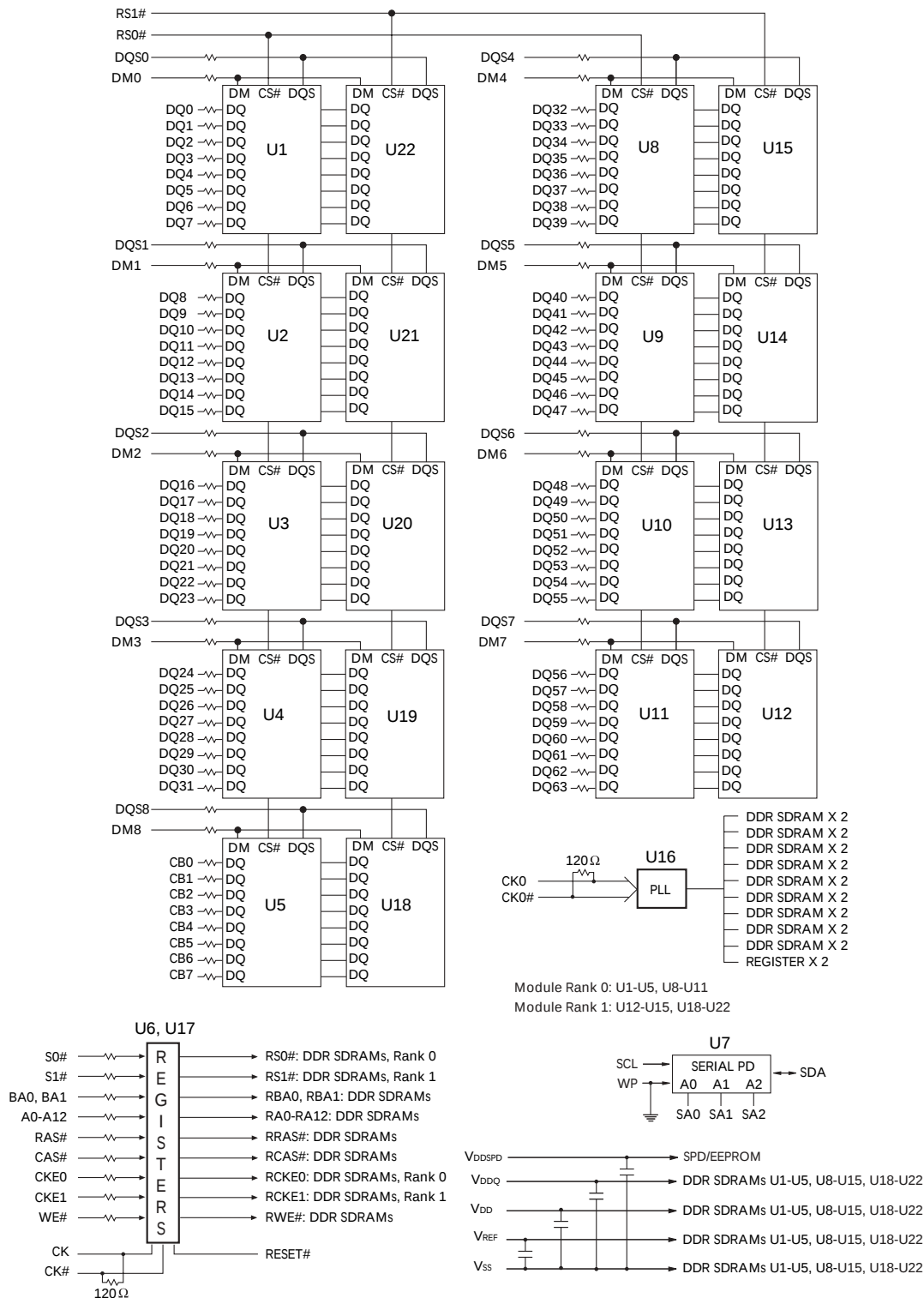
Figure 4: VLP DIMM Functional Block Diagram
