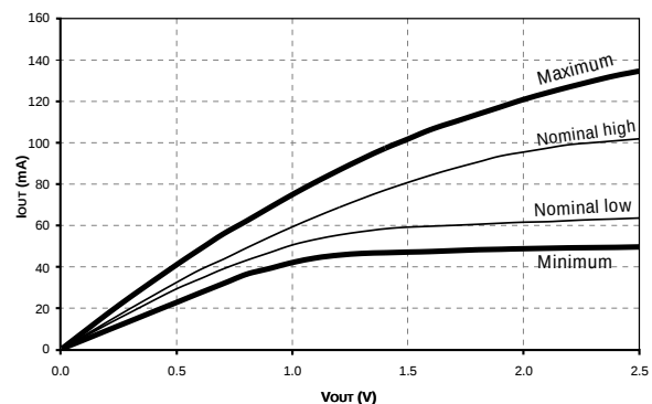
Figure 9: Pull-Up
