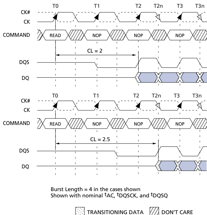
Figure 5: CAS Latency Diagram
