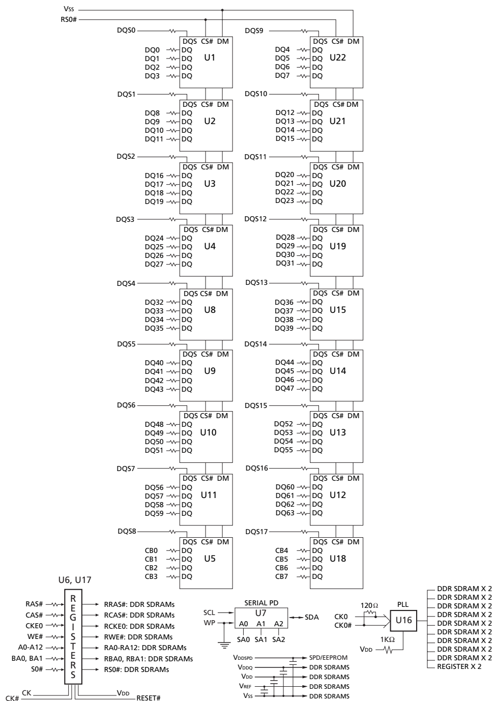
Figure 3: Functional Block Diagram – Very Low-Profile PCB
