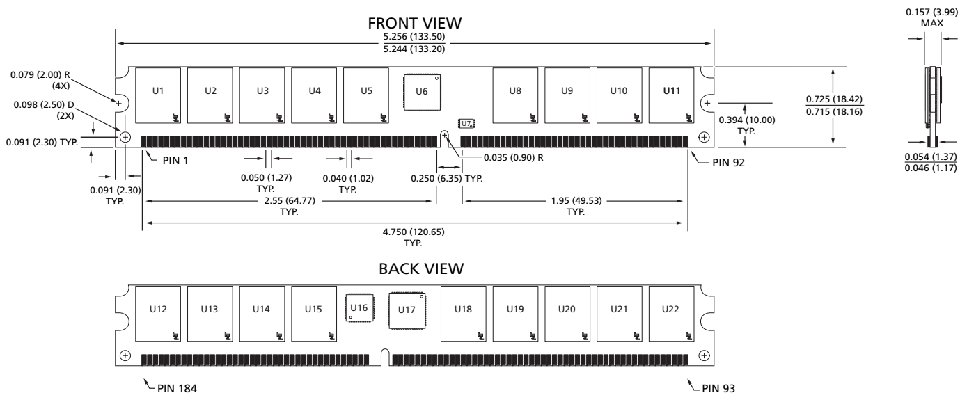
Figure 16: 184-Pin VLP DDR DIMM Dimensions
