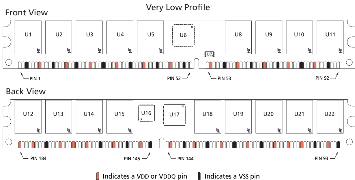
Figure 2: Pin Locations
