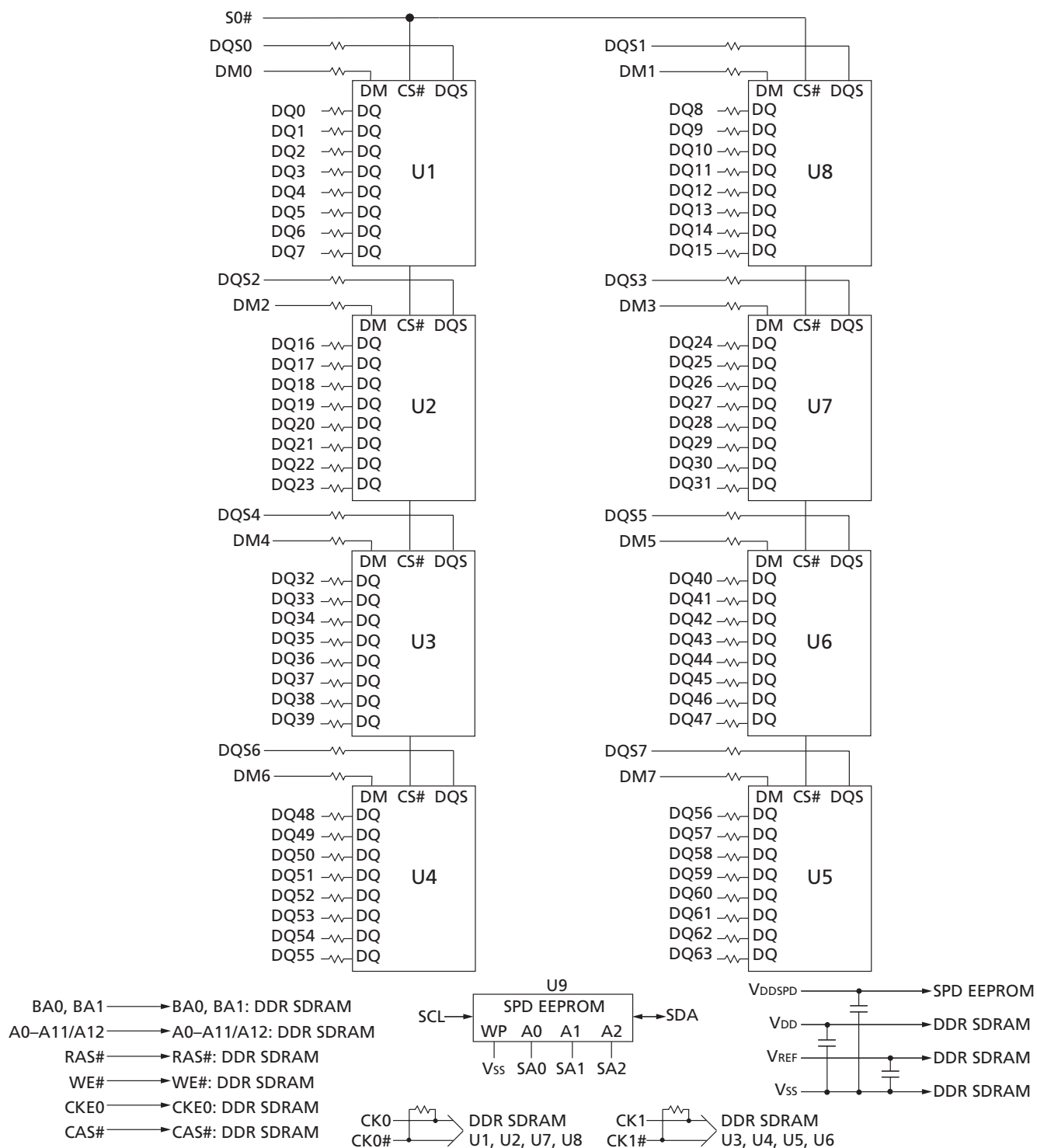
Figure 3: Functional Block Diagram – Layout 2 (128MB, 256MB, 512MB)
