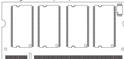
Figure 1: 200-Pin SODIMM (MO-224)
