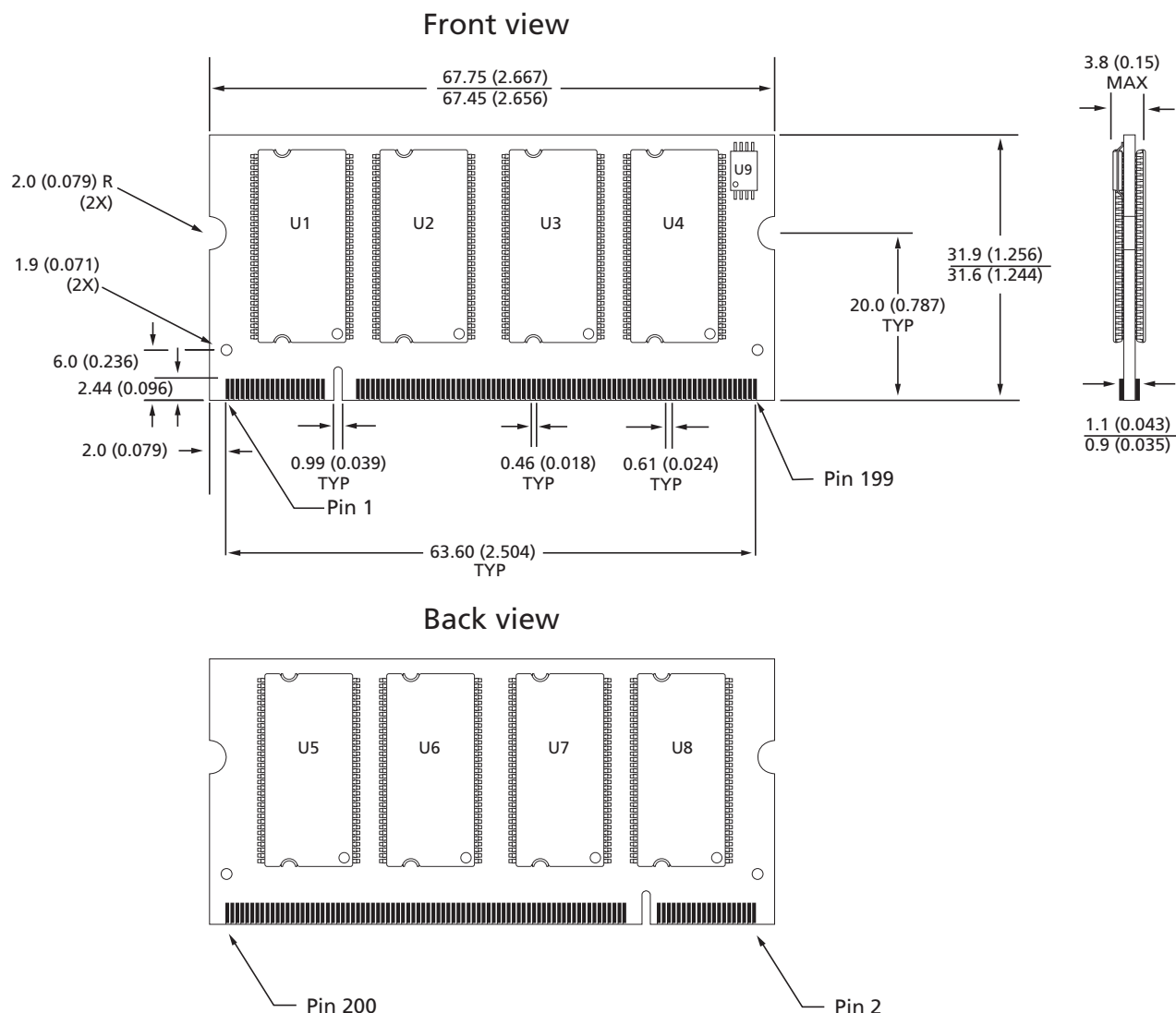
Figure 5: 200-Pin SODIMM – Layout 2 (128MB, 256MB, 512MB)
