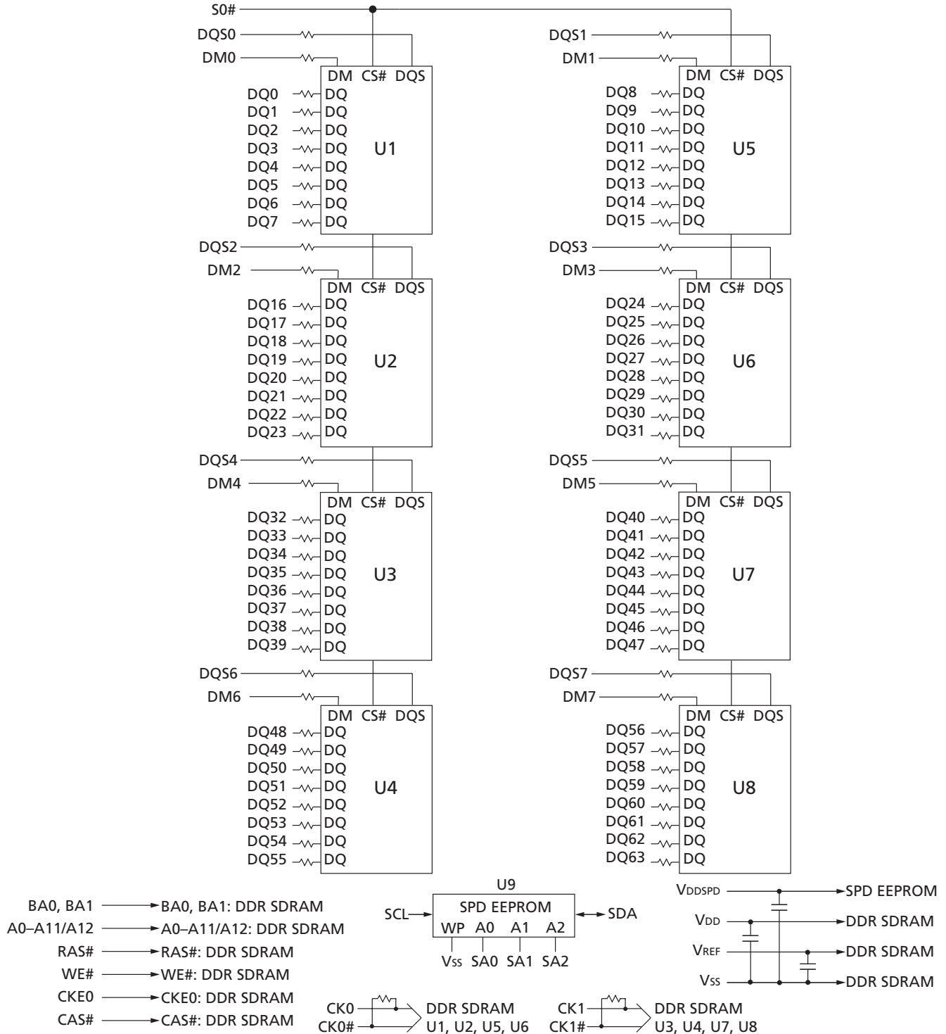
Figure 2: Functional Block Diagram – Layout 1 (128MB, 256MB)
