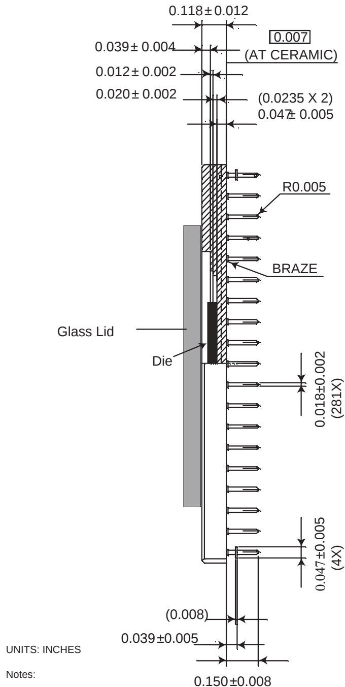
Figure 20: 280-Pin Ceramic PGA Package Side View
