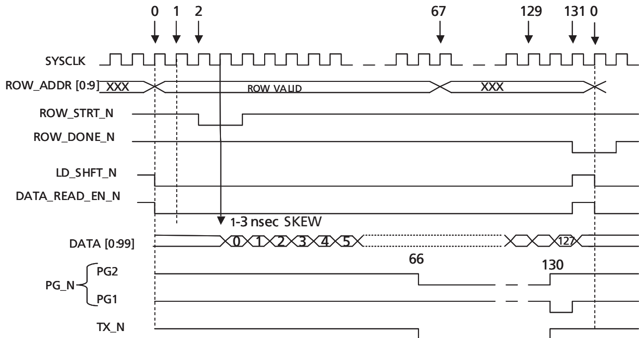
Figure 6: Timing Diagram For One Row
