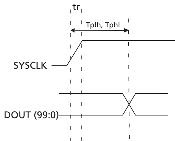
Figure 14: Clock to Data Propagation Delay
