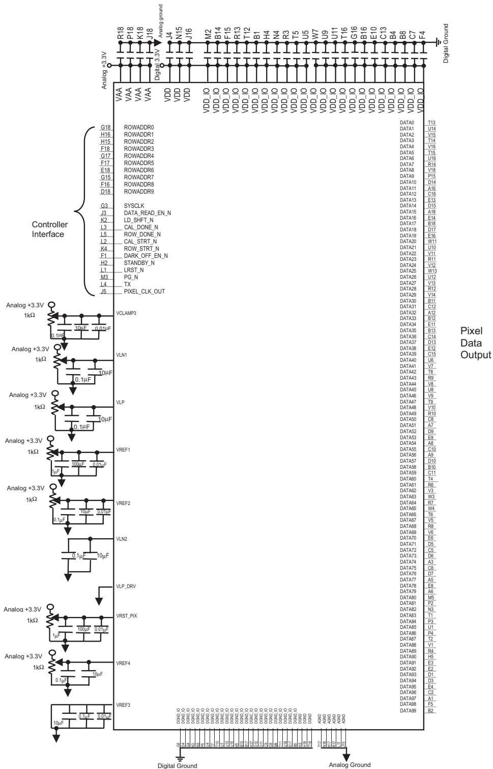
Figure 12: Board Connections
