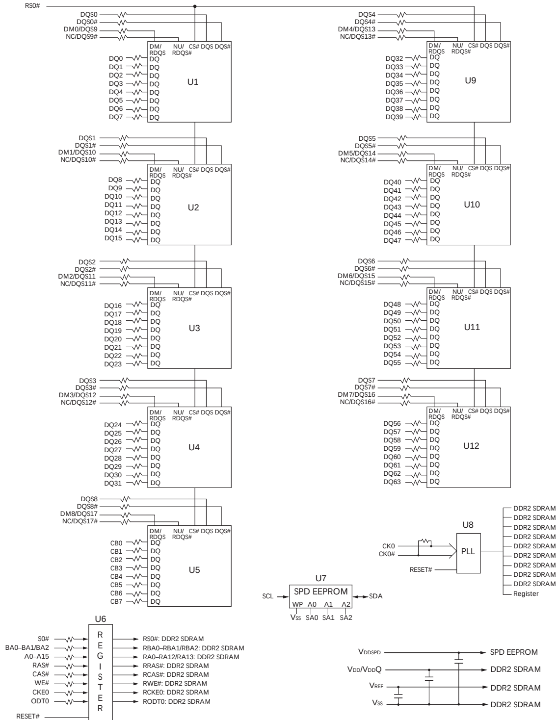
Figure 2: Functional Block Diagram – Raw Card A Non-Parity
