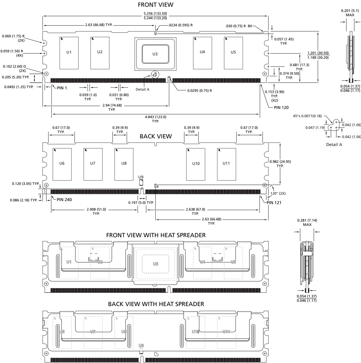
Figure 12: 240-pin DDR2 FBDIMM Module Dimensions
