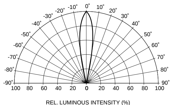
Fig. 4 Radiation Diagram
