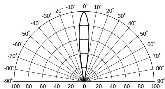
Fig. 4 Radiation Diagram
