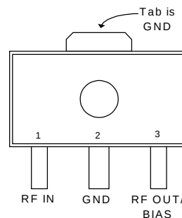
PK PACKAGE (Top View)
