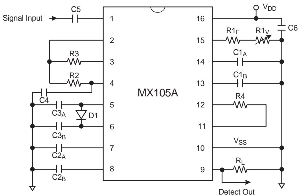
Figure 2: Recommended External Components
