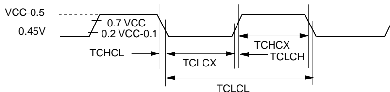
Figure 9. Clock Signal Waveform for ICC Tests in Active and Idle Modes. TCLCH = TCHCL = 5 ns
