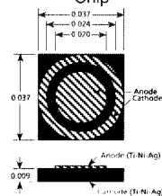
Figure 2 Chip
