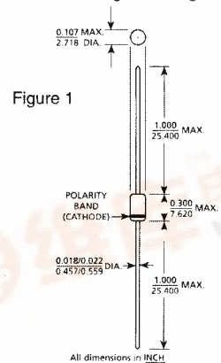
Package Drawing
