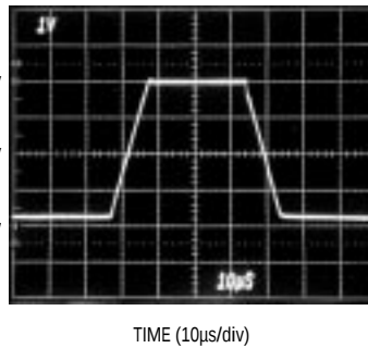
LARGE-SIGNAL TRANSIENT RESPONSE ( V_S = 5V, 0V )
