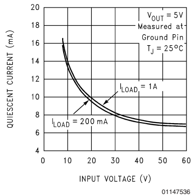
Quiescent Current
