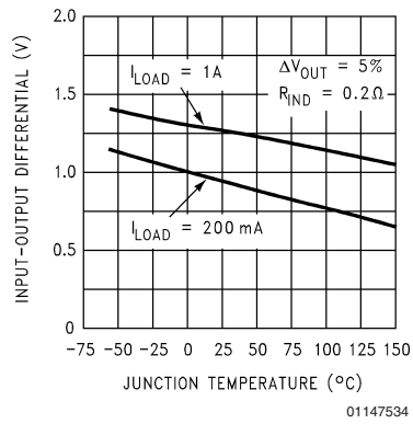
Dropout Voltage
