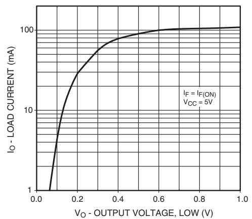
Figure 5. Load Current vs. Output Voltage
