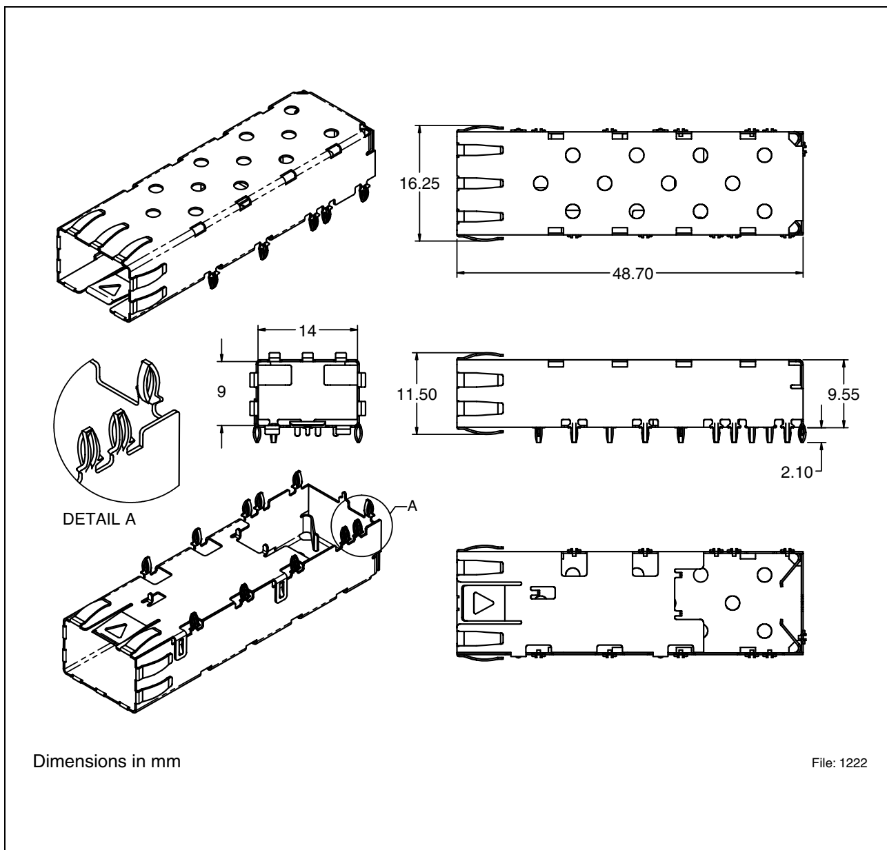
Figure 9 V23838-S5-N1-BB
