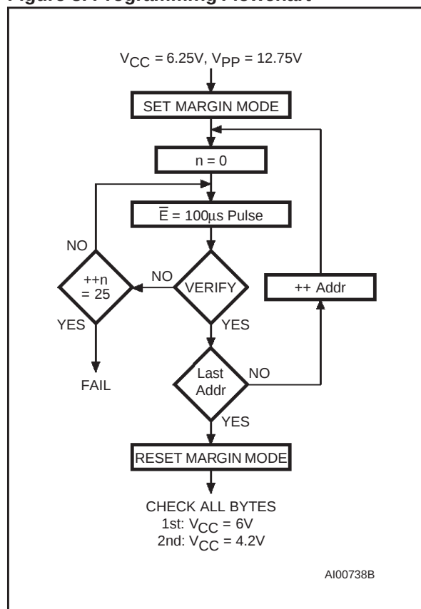
Figure 8. Programming Flowchart
