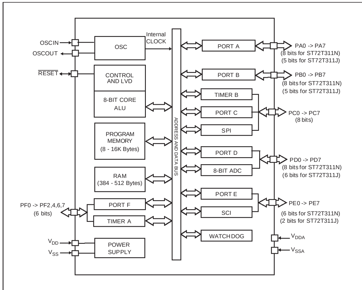
Figure 1. ST72T311 Block Diagram
