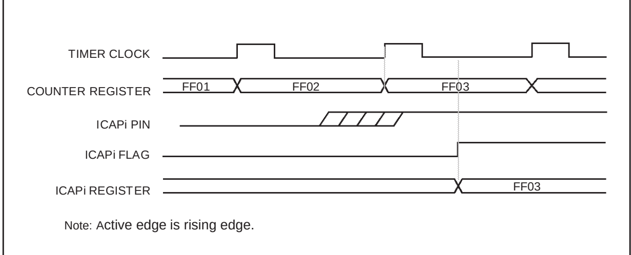
Figure 28. Input Capture Timing Diagram
