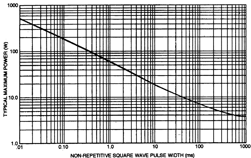
FIGURE 2 TRANSIENT SURGE CAPABILITY
