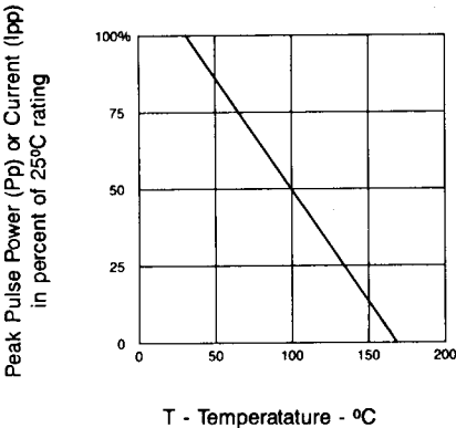
Figure 4. Derating Curve
