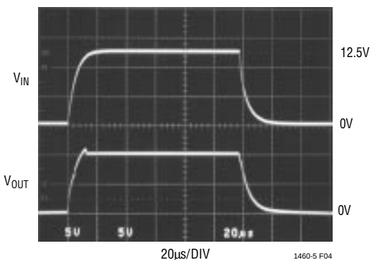
Figure 5. C_{IN} = 0.1\mu F
