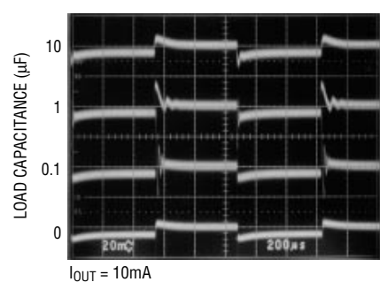
Transient Responses
