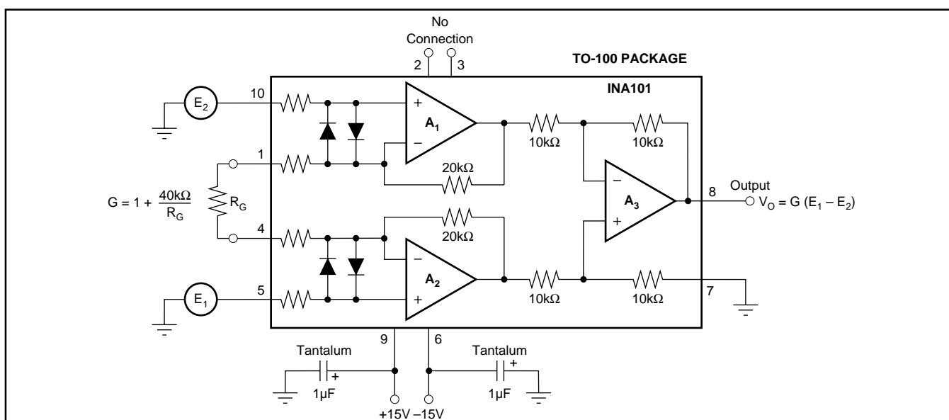
FIGURE 1. Basic Connections.
