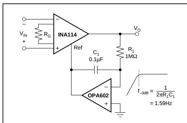
FIGURE 12. AC-Coupled Instrumentation Amplifier.
