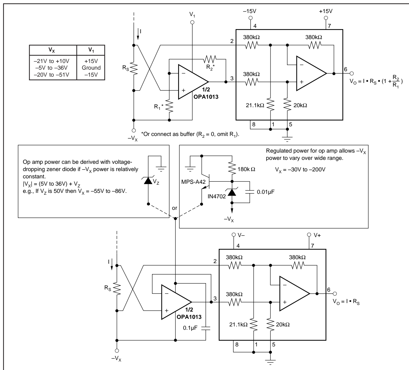
FIGURE 7. Current Sensing with Input Buffer.
