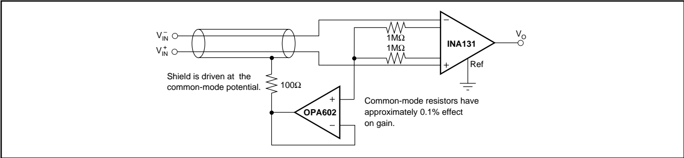
FIGURE 4. Shield Driver Circuit.
