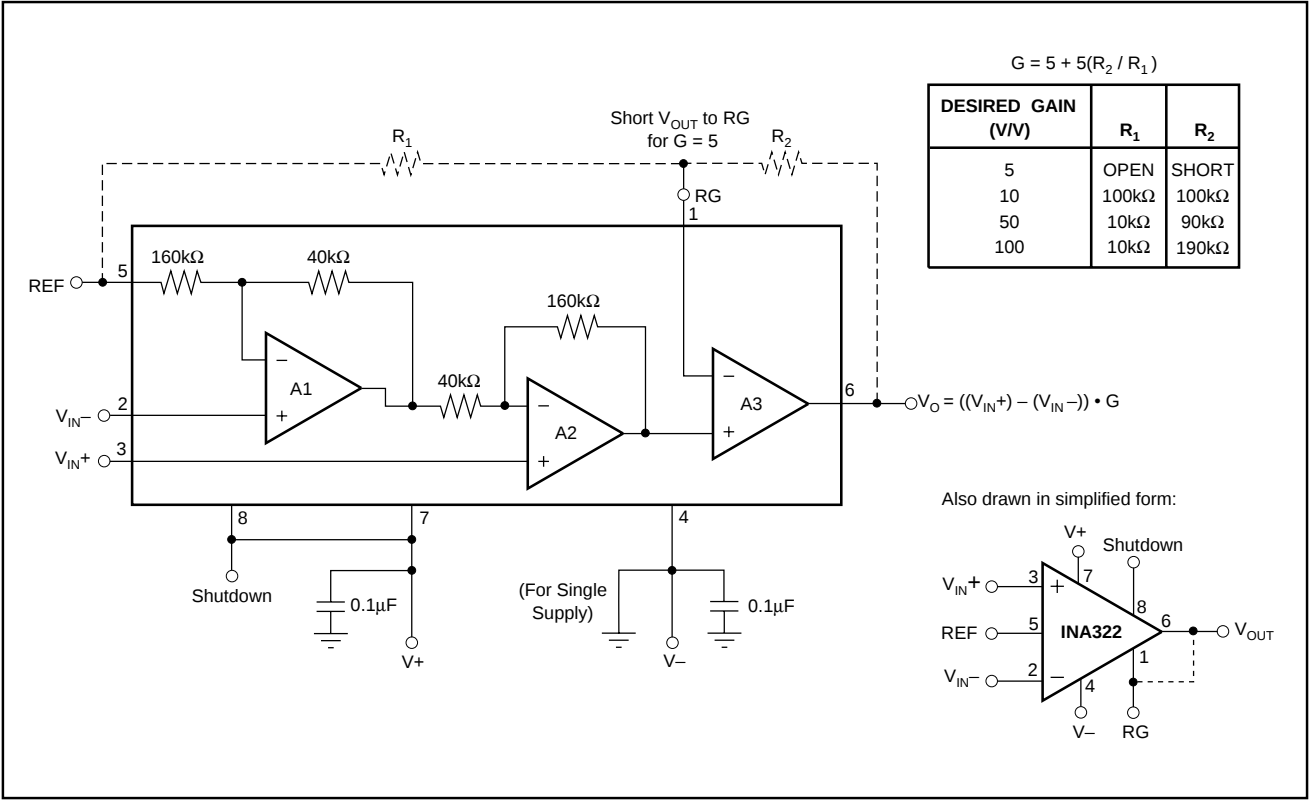
FIGURE 1. Basic Connections.
