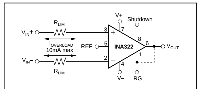
FIGURE 7. Input Protection.
