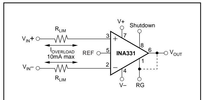
FIGURE 7. Sample Output Buffering Circuit.
