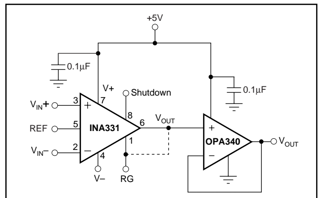
FIGURE 5. Output Buffering Circuit. Able to drive loads as low as 600\Omega .
