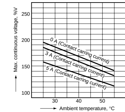
6.-(2) Ambient temperature vs Max. continuous voltage Sample: NC2D-P-DC110 V (2c slim single side stable), NC4D-P-DC24 V (4c slim single side stable)
