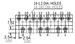
PC board pattern (Copper-side view)
