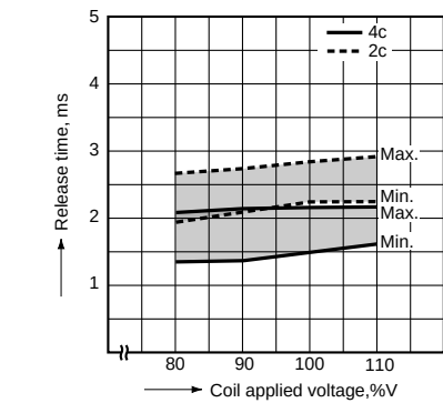
4. Release time for single side stable
