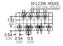
PC board pattern (Copper-side view)
