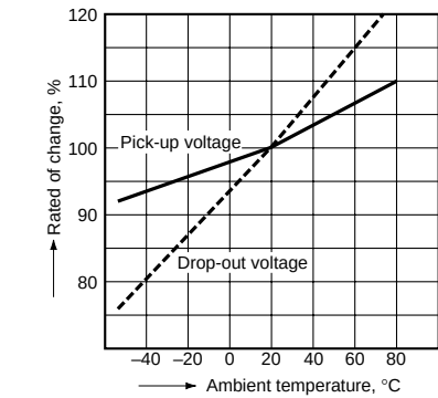
5. Rate of change of pick-up and drop-out voltage 2 Form C single side stable
