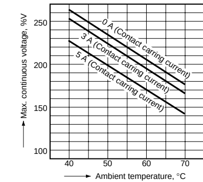
6.-(1) Ambient temperature vs Max. continuous voltage Sample: NC2D-P-DC24 V (2c slim single side stable)
