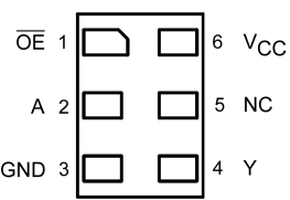
Pad Assignments for MicroPak
