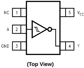
Pad Assignments for MicroPak
