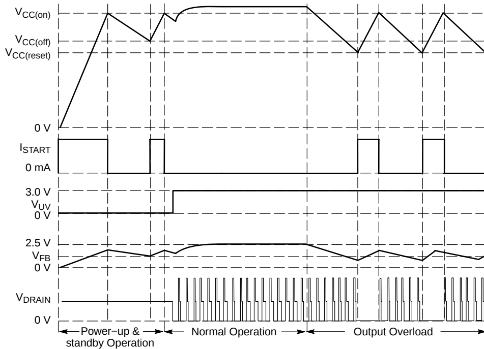
Figure 3. Auxiliary Winding Operation with Output Overload Timing Diagram
