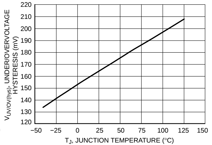
Figure 17. Line Under/Overtolerance Hysteresis vs. Junction Temperature
