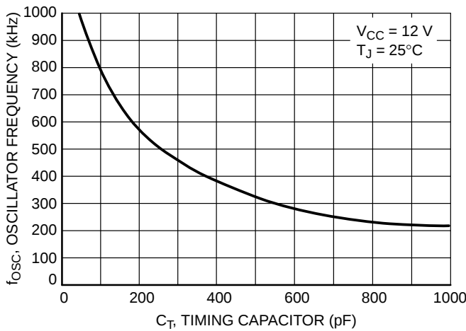
Figure 18. Oscillator Frequency vs. Timing Capacitor
