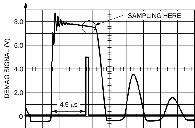
Figure 23. A Voltage Sample is Taken 4.5 \mu s After the Turn-Off Sequence
