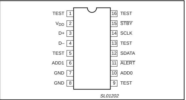
Figure 1. Pin configuration
