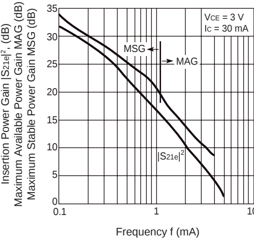
INSERTION POWER GAIN, MAG, MSG vs. FREQUENCY
