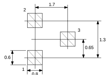
OUTLINE 30 RECOMMENDED P.C.B. LAYOUT
