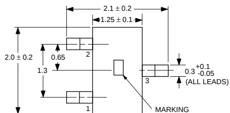
OUTLINE 30 (SOT-323)
