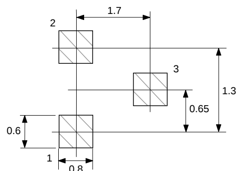
PACKAGE OUTLINE 30 RECOMMENDED P.C.B. LAYOUT
