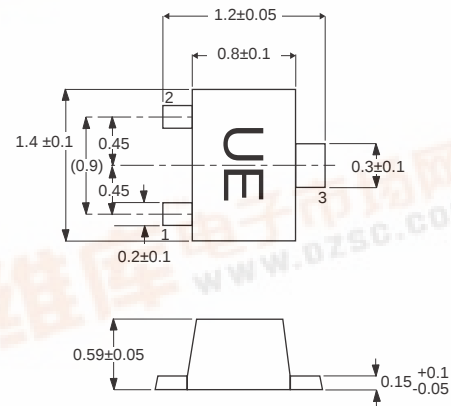
PACKAGE OUTLINE M03
