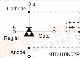
Figure 1. Equivalent Circuit
