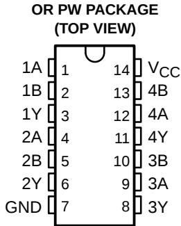
SN54AHCT08 ... J OR W PACKAGE SN74AHCT08 ... D, DB, DGV, N, NS, OR PW PACKAGE
