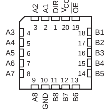
SN54AHCT245 . . . FK PACKAGE (TOP VIEW)
