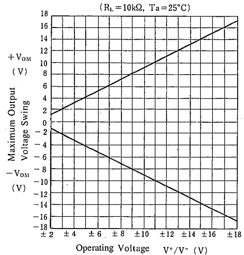
Maximum Output Voltage Swing vs. Operating Voltage
