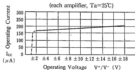
Operating Current vs. Operating Voltage
