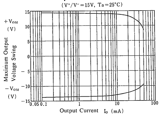
Maximum Output Voltage Swing vs. Output Current
