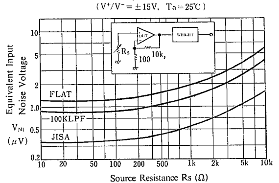
Equivalent Input Noise Voltage
