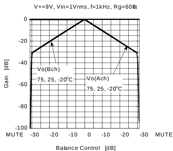
Gain vs Balance Control
