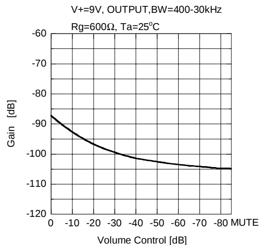
Output Noise vs Volume Control
