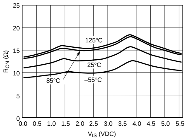
Figure 23. R_{ON} vs. Temp, V_{CC} = 5.5\text{ V}
