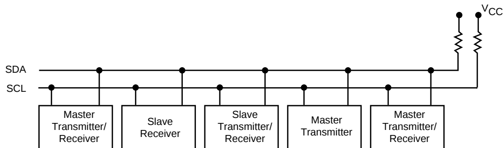
Typical System Configuration (Figure 11).
