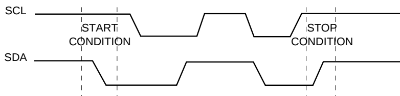
Start and Stop Definition (Figure 2).
