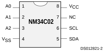
SO (M8) and TSSOP (MT8) Package
