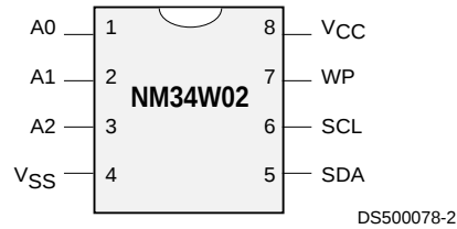
SO (M8) and TSSOP (MT8) Package
