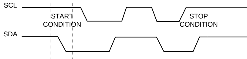
Start and Stop Definition (Figure 2).
