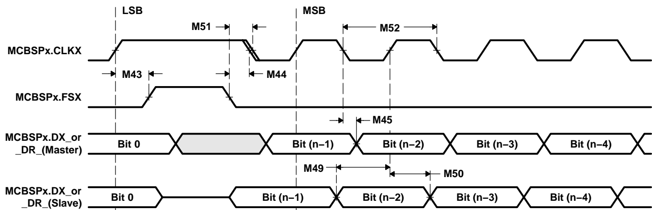
Figure 5–38. McBSP Timings as SPI Master or Slave: CLKSTP = 10b, CLKXP = 1
