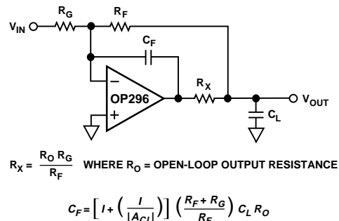
Figure 40. In-the-Loop Compensation Technique for Driving Capacitive Loads
