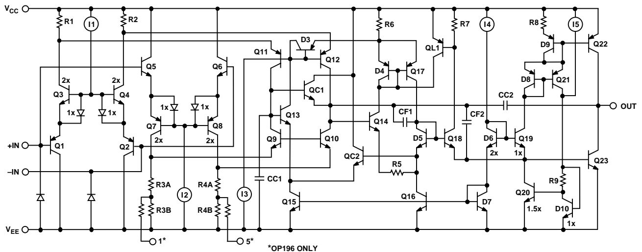
Figure 26. Simplified Schematic
